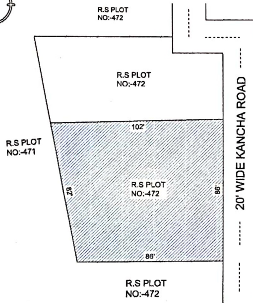
LAYOUT MAP Scale :- 1"=50'
