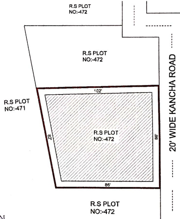
SITE PLAN Scale :- 1"=50'
